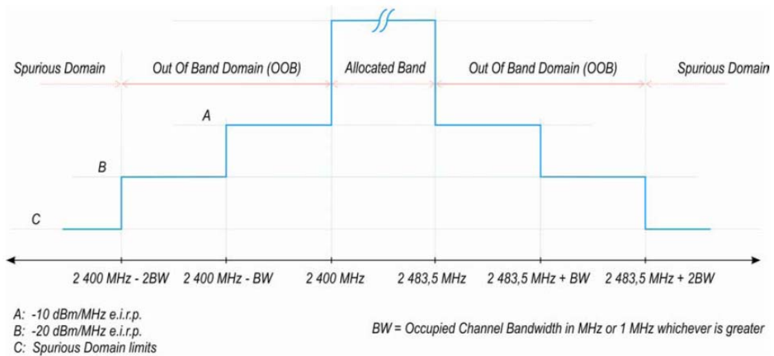
Figure 3: Transmit mask
