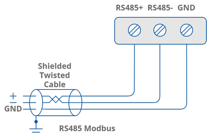
Figure 6. Communication bus connection
