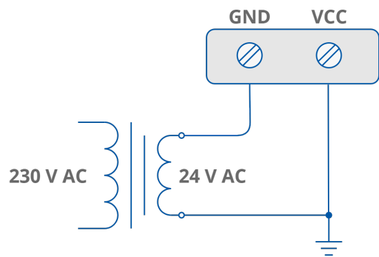
Figure 5. AC power connection
