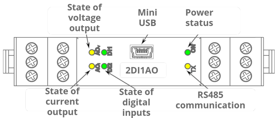
Figure 2. Indicators
