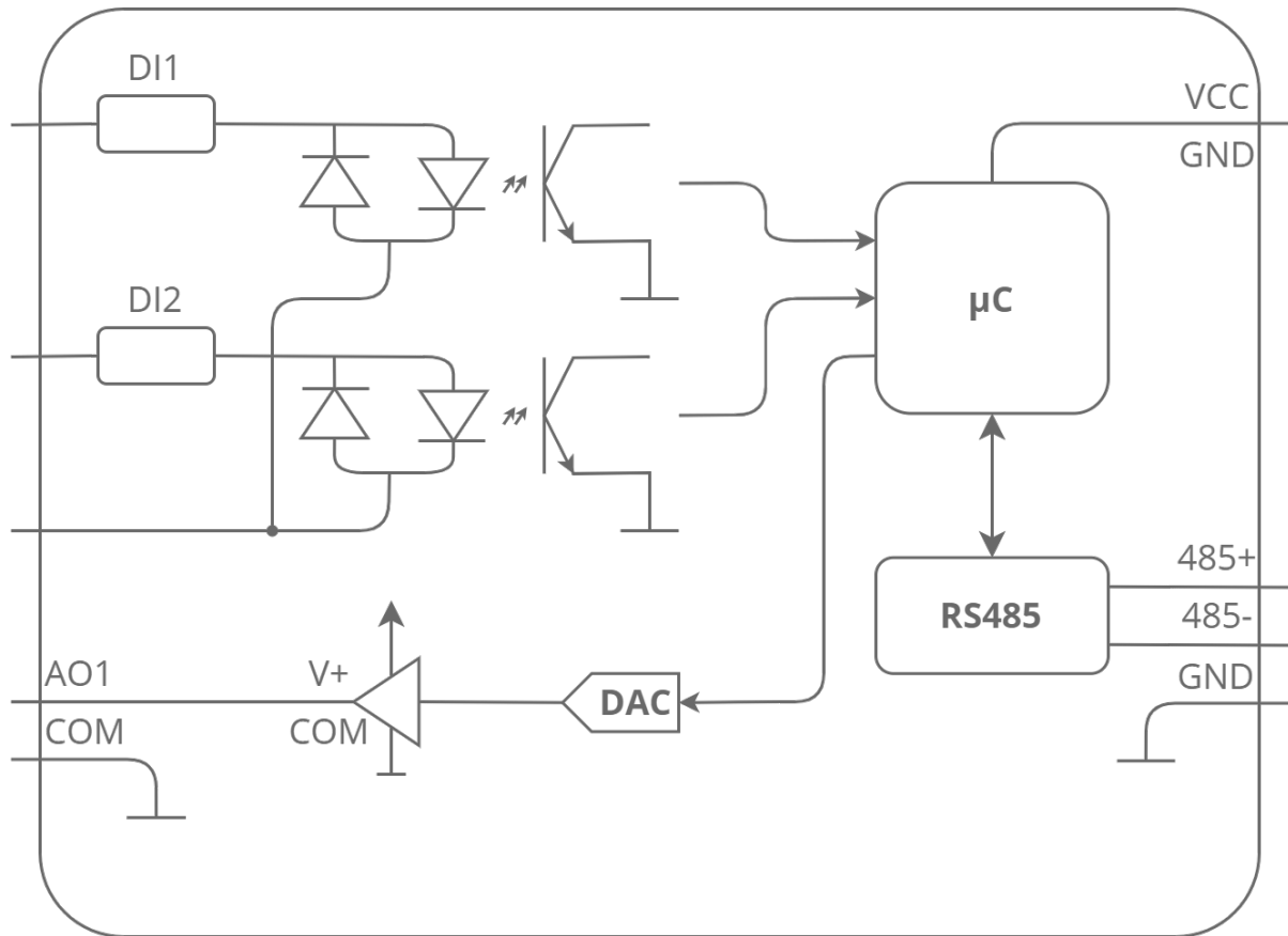
Figure 3. Block diagram
