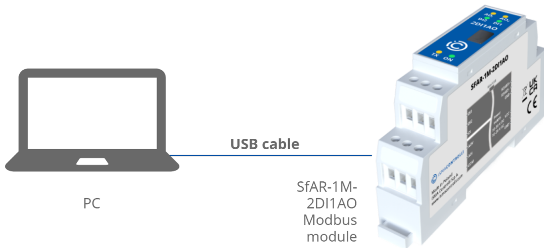
Figure 10. PC connection
