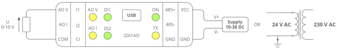
Figure 7. Connection of voltage output
