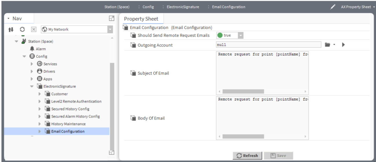
Figure 8 Email Configuration
