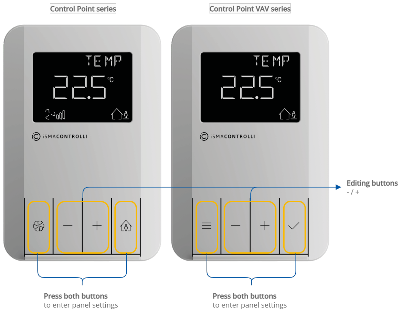
Figure 24. Editing settings
