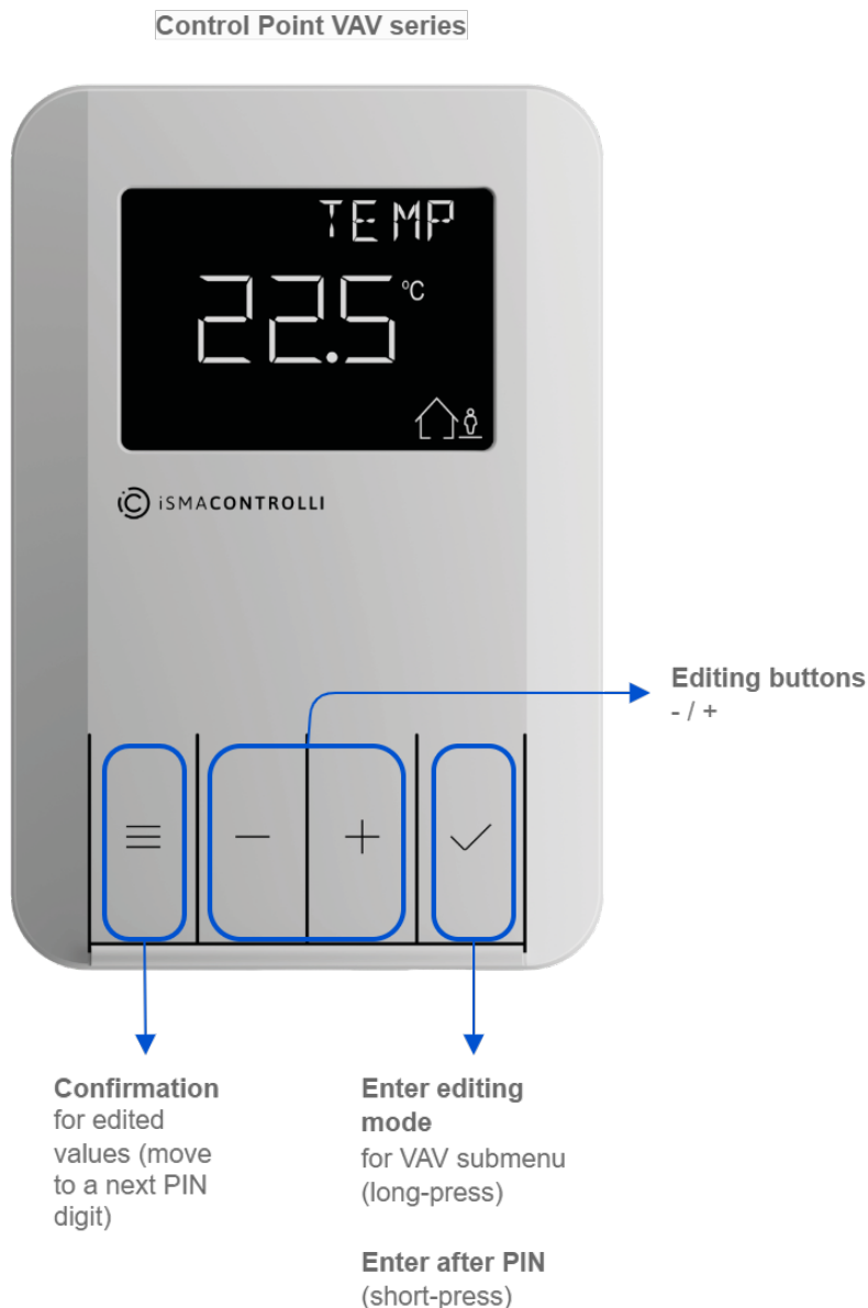
Figure 23. Editing VAV submenu
